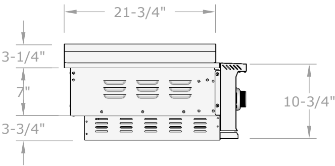
BACK VIEW (LEFT) SCALE 1:14
